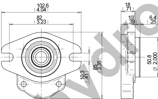
S0 SAE AA 2 bolts With shaft code 51-80
