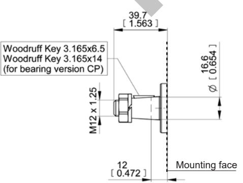
code 28 Max torque 130 Nm (1151 lbf in) Tapered 1:8
