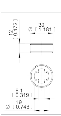
code 03 Max torque 70 Nm (620 lbf in) Tang drive for electric motors Without shaft seal
