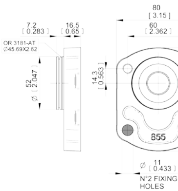
B2 German standard With shaft code 03
