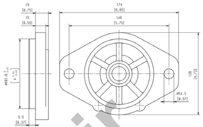
S3 SAE B 2 bolts With shaft code 55
