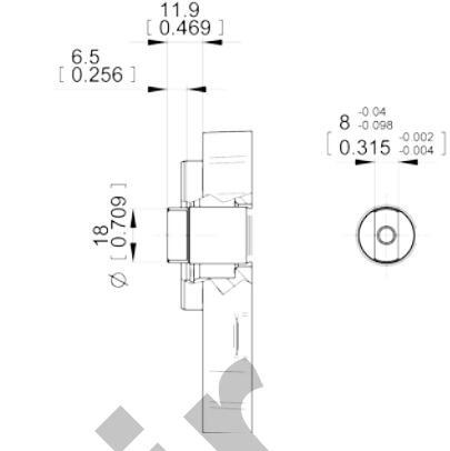
code 04 Max torque 70 Nm (620 lbf in) Tang drive
