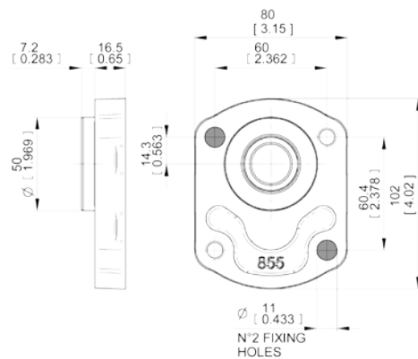
B5 German standard With shaft code 25-62-04
