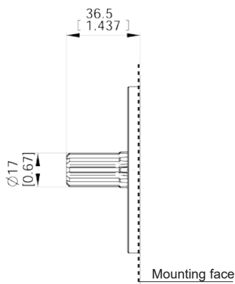
code 53 Max torque 125 Nm (1106 lbt in) SAE A 10T-16/32DP Ansi B92 1a 1976
