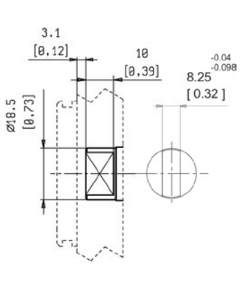
code 02 Max torque 70 (620 lbf in) Tang drive for engine driven For flange K1 without shaft seal
