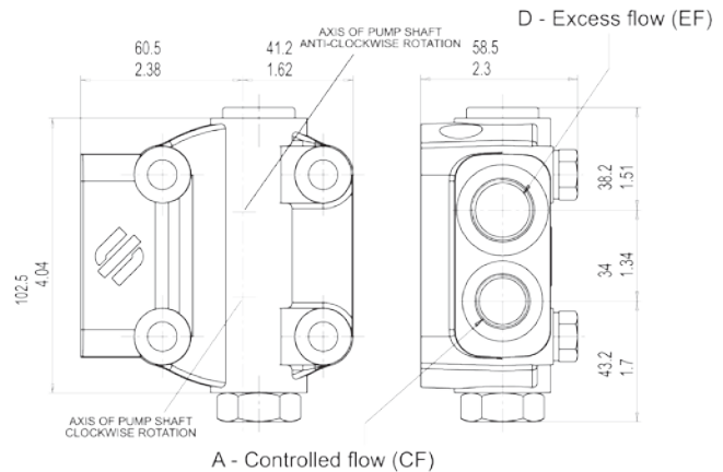
VP1 - VPS1 SIDE PORTS
