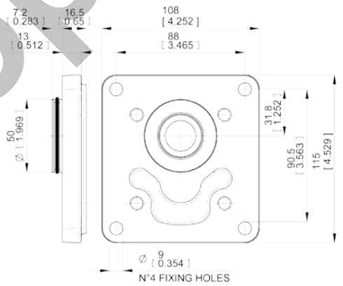
C1 4 bolts for Iveco engines With shaft code 62
