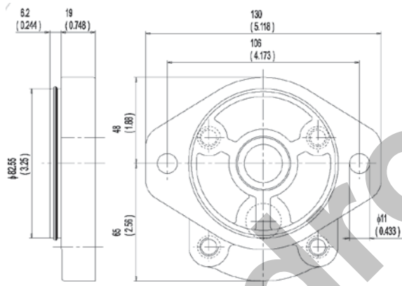
S6 SAE A 2 bolts (with O-ring on the centering collar) With shaft code 52-54-82-85
