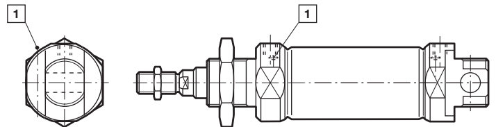
1 Cushion screw
