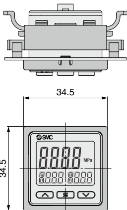
B Panel mount adapter (Part no.: ZS-46-B)
