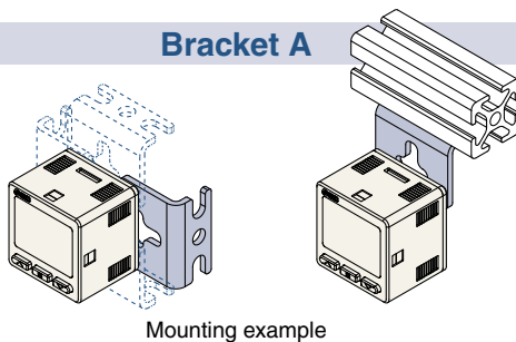
Mounting example
