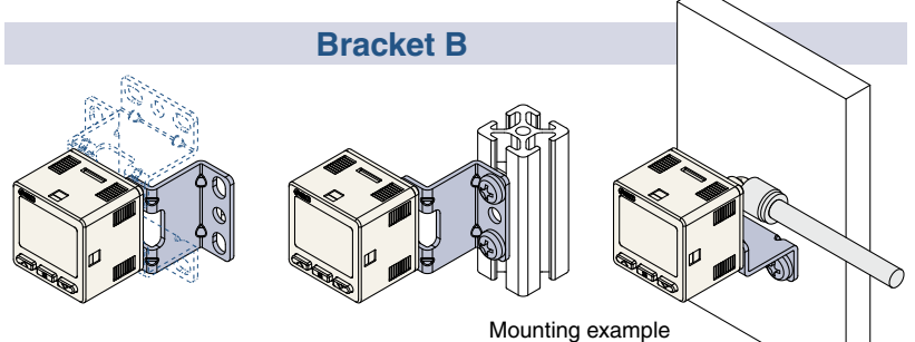
Mounting example
