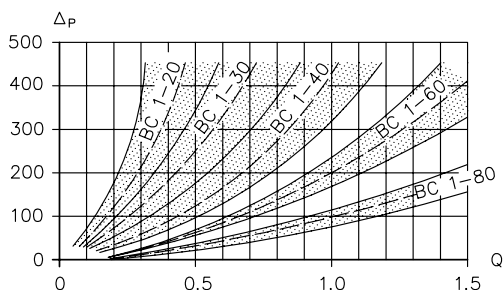
Q flow rate (lpm); \Delta p flow resistance (bar)
