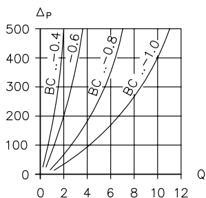
Q flow rate (lpm); \Delta p flow resistance (bar)
